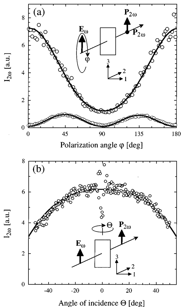
FIG. 3. SHG intensity as a function of the polarization angle and the angle of incidence. The PEBA thin film with a thickness of 180 nm was deposited on fused silica at a substrate temperature of 100 °C and a deposition rate of 5 nm/min.
