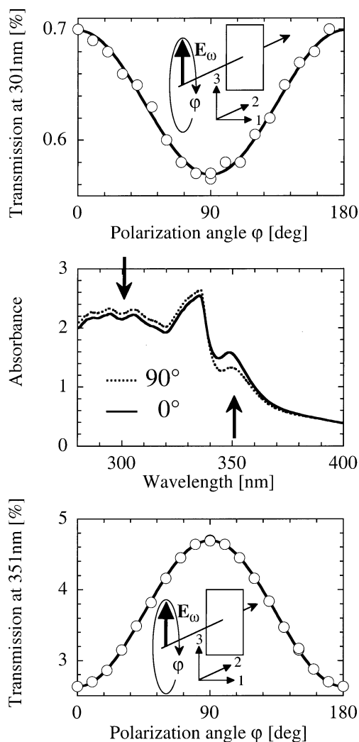
FIG. 2. Transmission measurements of UV light for a 270-nm-thick PEBA film on fused silica (Suprasil ® ) deposited at a substrate temperature of 100 °C and a deposition rate of 5.5 nm/min. The upper and lower images represent the transmission vs polarization angle at a wavelength of 301 and 351 nm, respectively, following perfectly a sine and shifted to each other by 90°. The central part shows the anisotropy of the absorbance.
