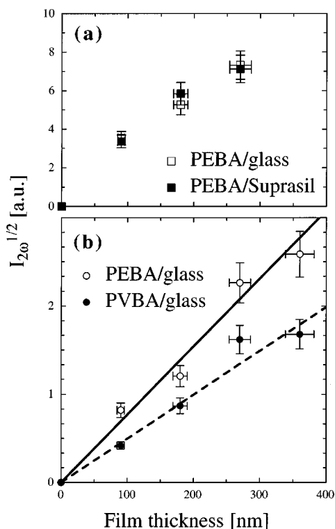
FIG. 4. Variation of the square root of the SHG intensity with the film thickness. (a) PEBA on glass and fused silica grown at a substrate temperature of 100 °C and a deposition rate of (4 \pm 1) nm/min; (b) PEBA and PVBA on glass deposited at a substrate temperature of 30 °C and a rate of (4 \pm 1) nm/min.
